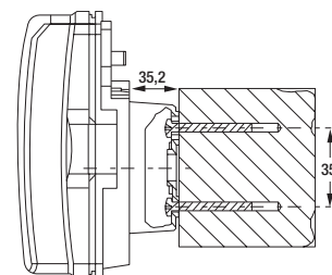
Fixation murale
