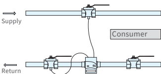
Symmetrical sensor installation for Celsius C5
