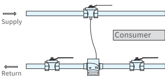
Asymmetrical sensor installation for Celsius C5 with one temperature sensor integrated in the flow sensor
